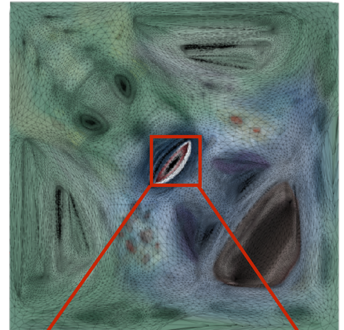
Texture image
